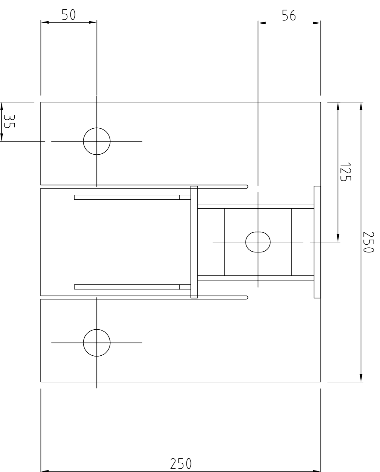
Baseplate Detail
