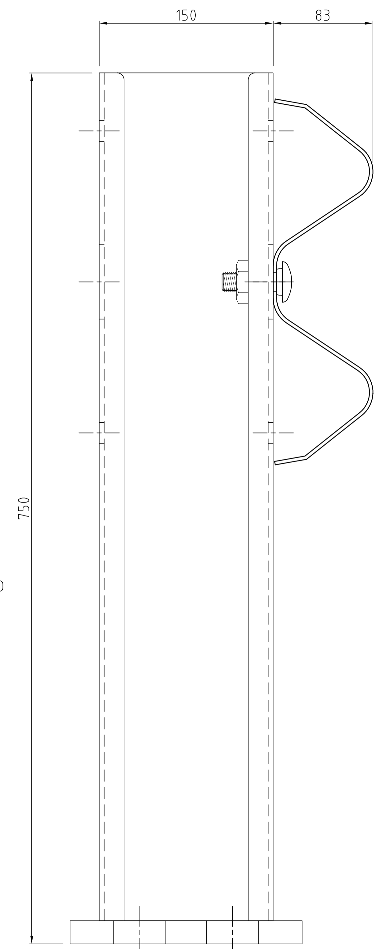
POST ELEVATION
