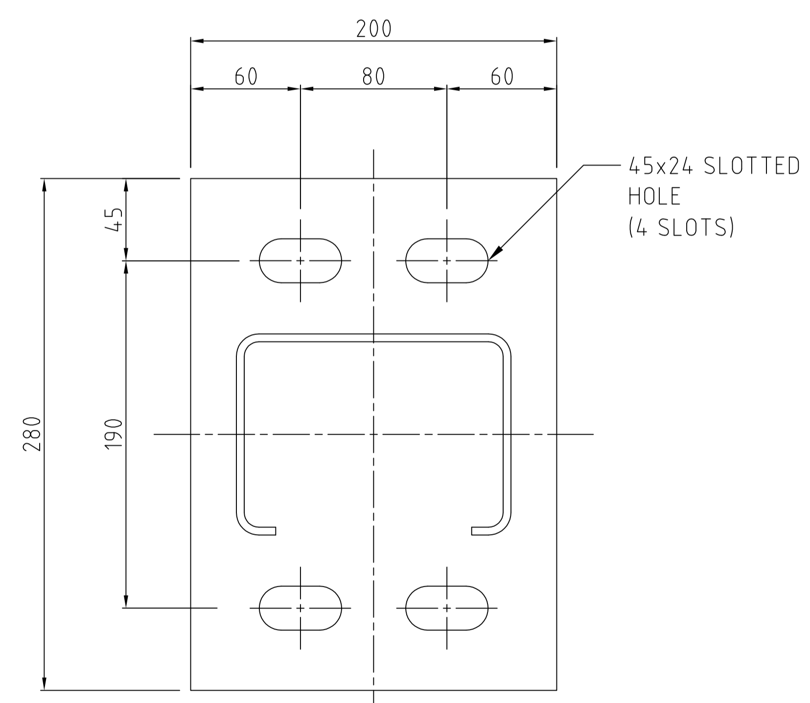
BASE PLATE DETAIL
