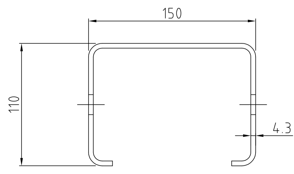
POST PLAN
