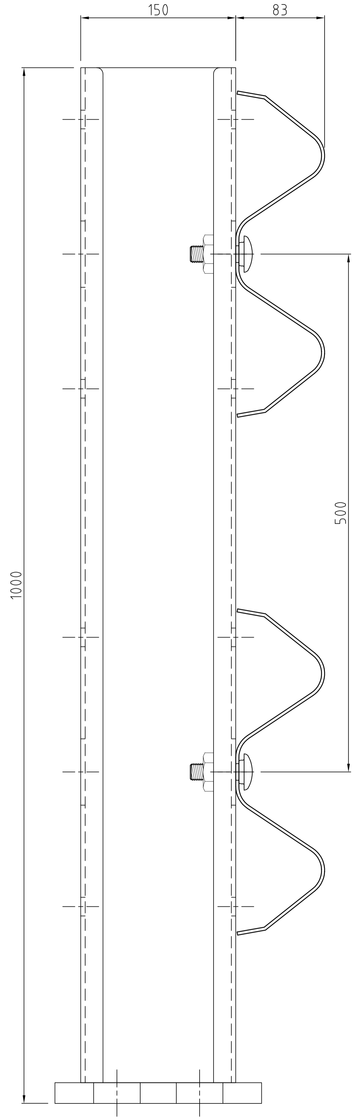
POST ELEVATION
