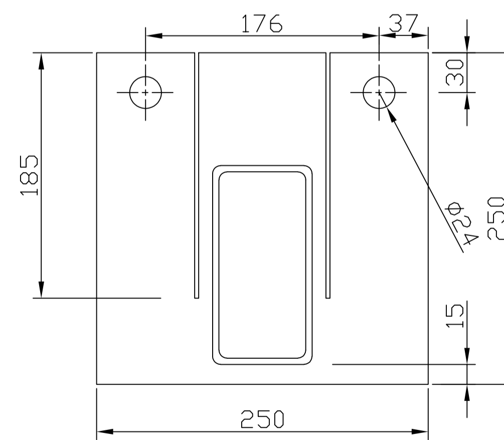
Baseplate Detail
