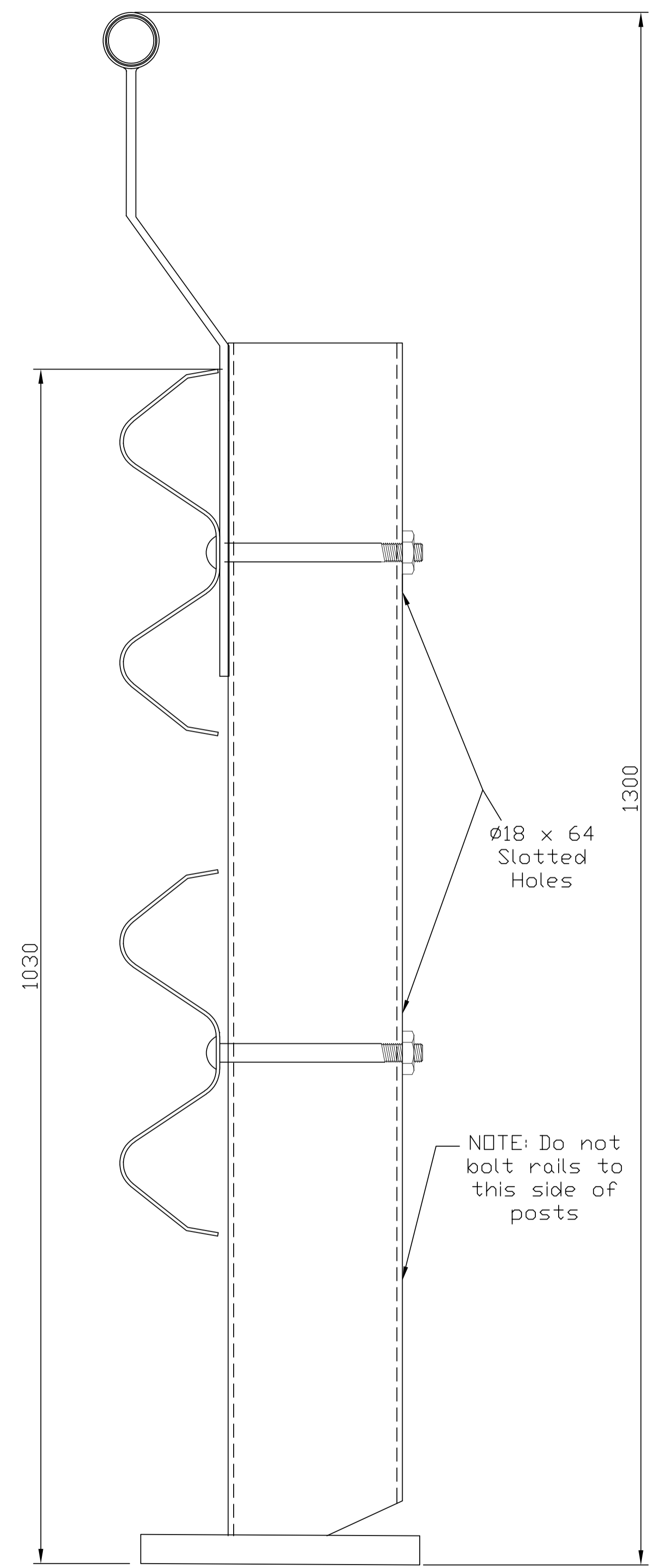
Elevation View
