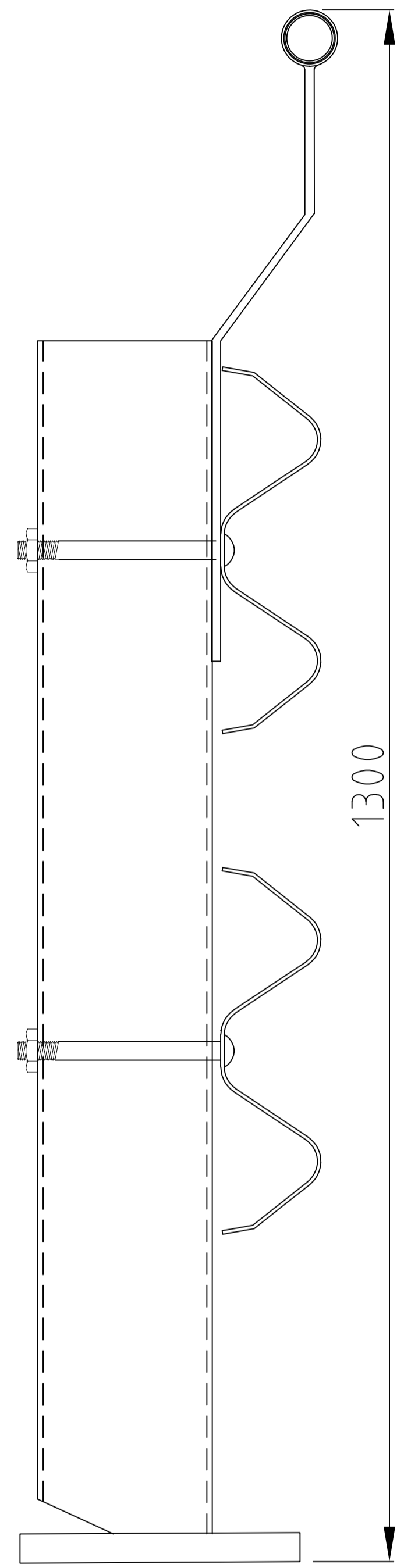
Rhino-Stop Truck Guard Type 3 Guardrail & Nearside Balustrade
