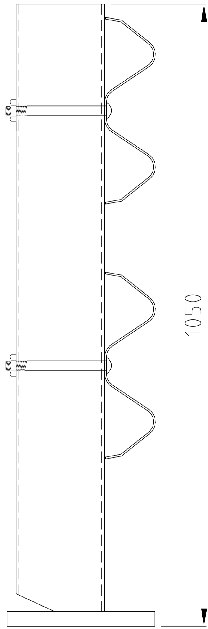
Rhino-Stop Truck Guard Type 1 Guardrail
