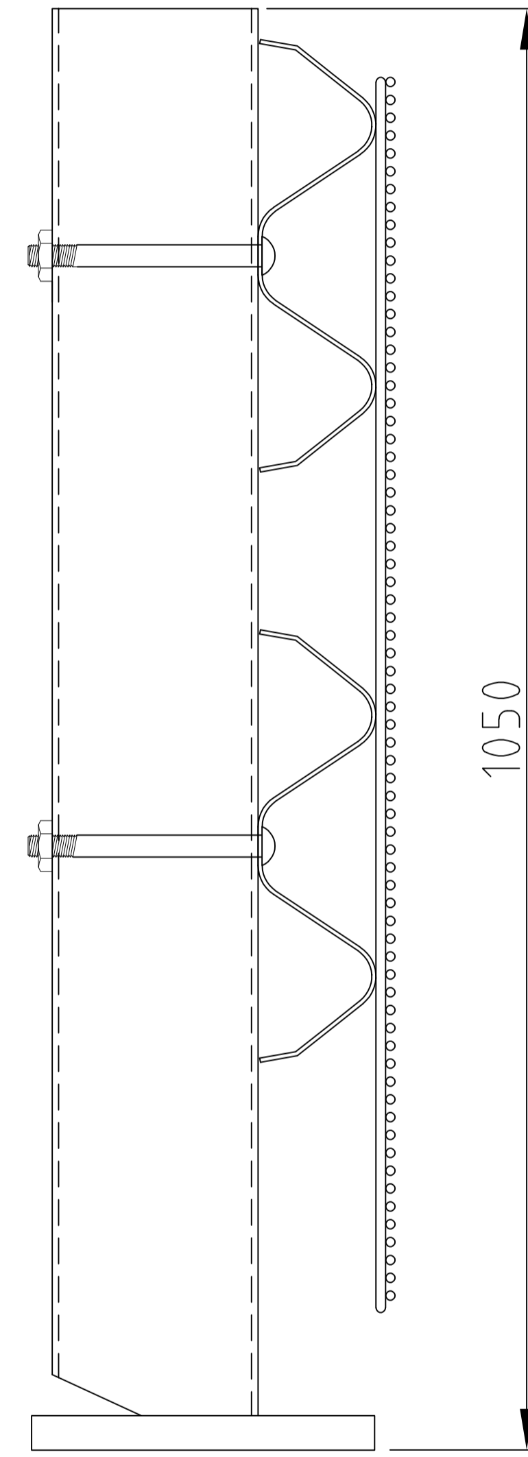
Rhino-Stop Truck Guard Type 4 Guardrail Anti-Climb Mesh
