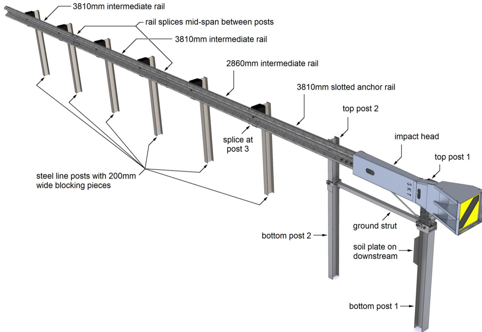
Figure 2: MSKT Component Identification (TL3)
