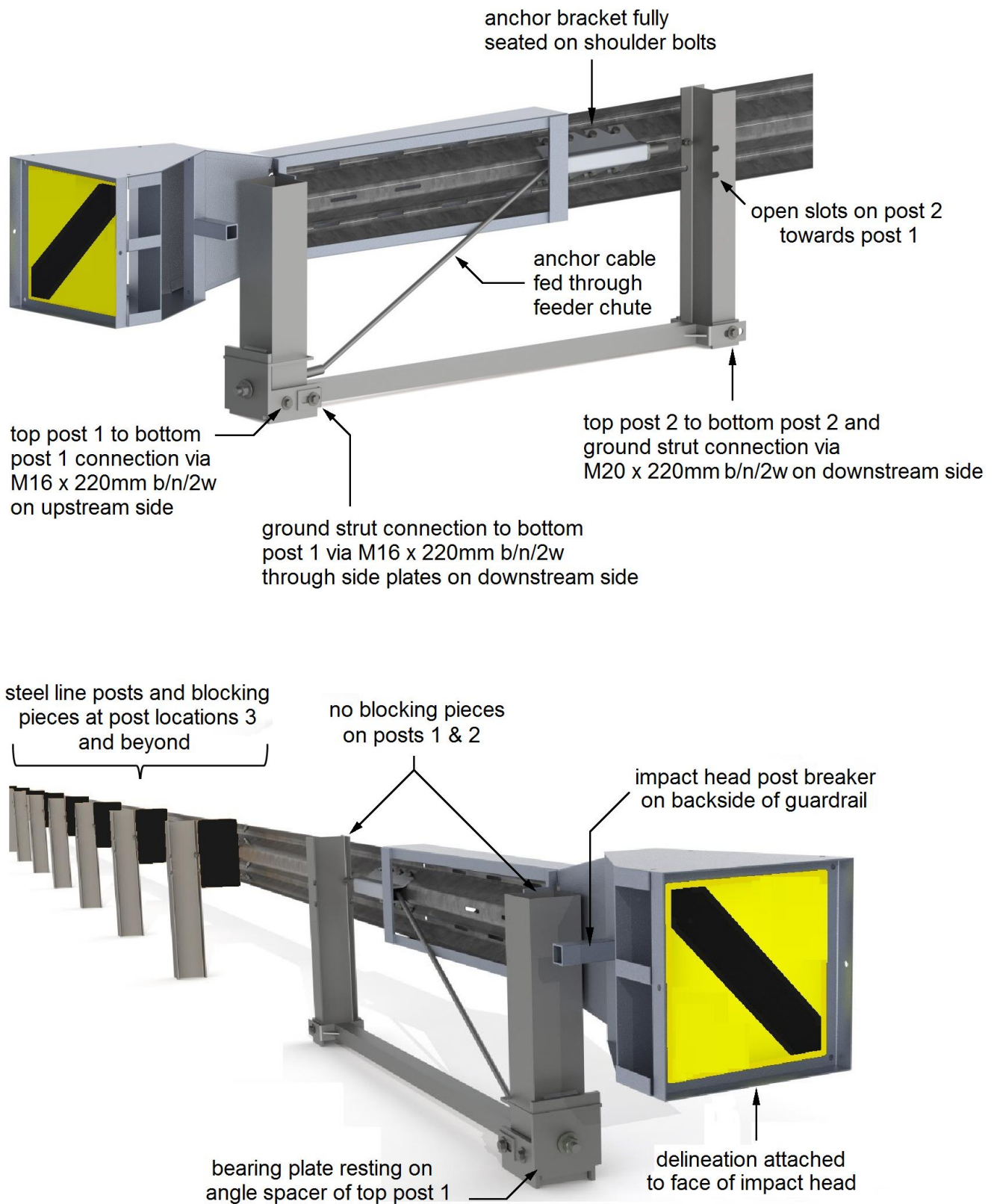
Figure 10: Cable Assembly and Impact Head Assembly Detail
