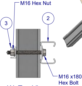
'A' Top View SCALE 1:10
