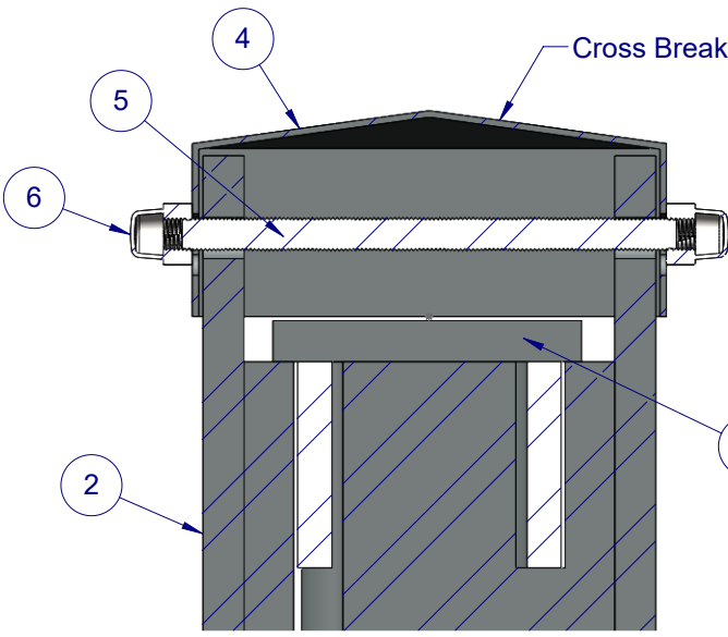
Section A - A Intermediate Post & Cap Connection Top Detail
