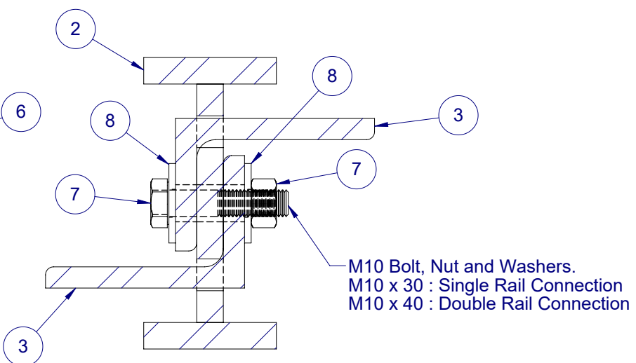
Section B - B Intermediate Post Connection Bottom Detail
