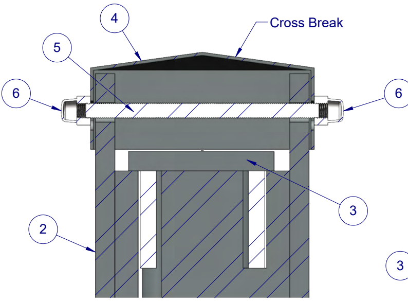
Section A - A Intermediate Post & Cap Connection Top Detail
