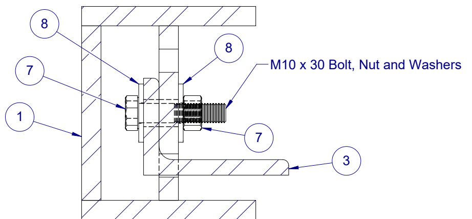
Section C - C End Post Connection Bottom Detail
