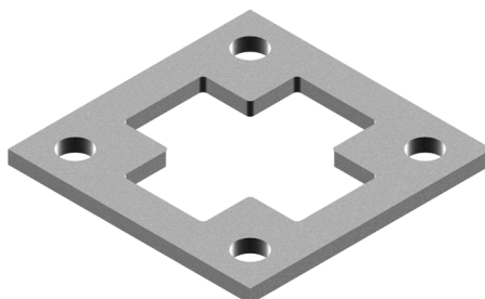
2110839SLM x 3 SL WIRE ROPE STE HDA BASEPLATE 180x180x10 4M20 130C.R.S
