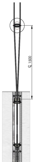
DETAIL A - PLAN VIEW END TERMINAL TO TRANSITION POSTS WIRE ROPE TRANSITION SCALE 1 : 20
