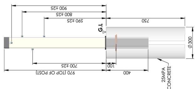
TYPICAL LINEPOST DETAIL ELEVATION VIEW SCALE 1 : 12
