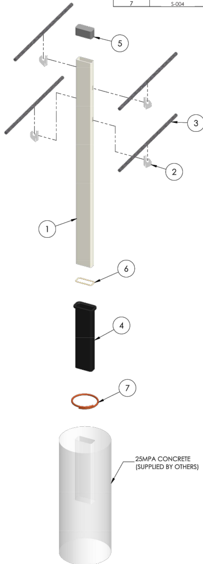
ISO EXPLODED VIEW SCALE 1:10
