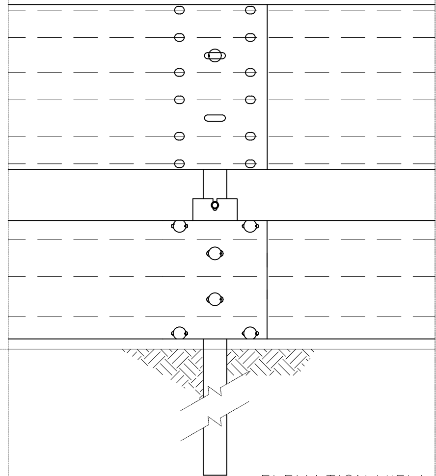
ELEVATION VIEW
