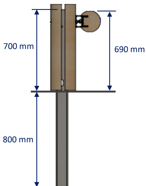
SIDE ELEVATION
