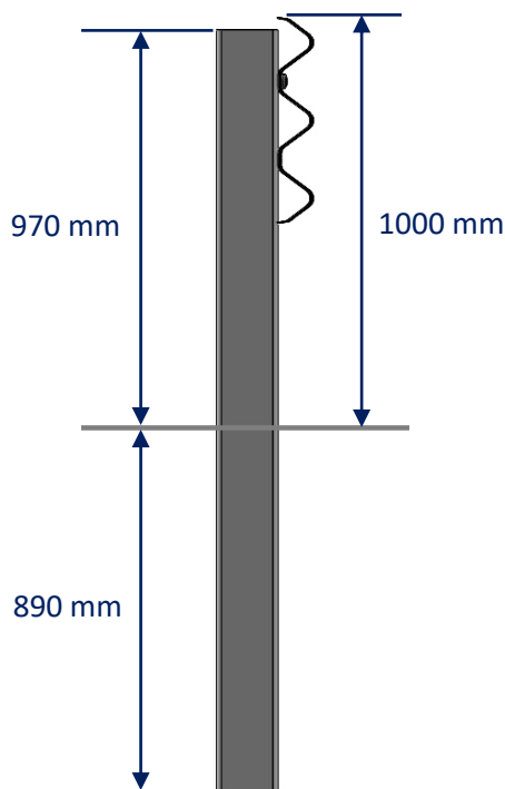
SIDE ELEVATION
