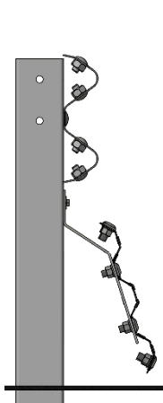
Attachment to Sentry W-Beam SIDE ELEVATION
