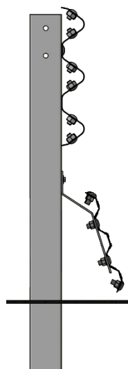
Attachment to Sentry Thrie-Beam SIDE ELEVATION
