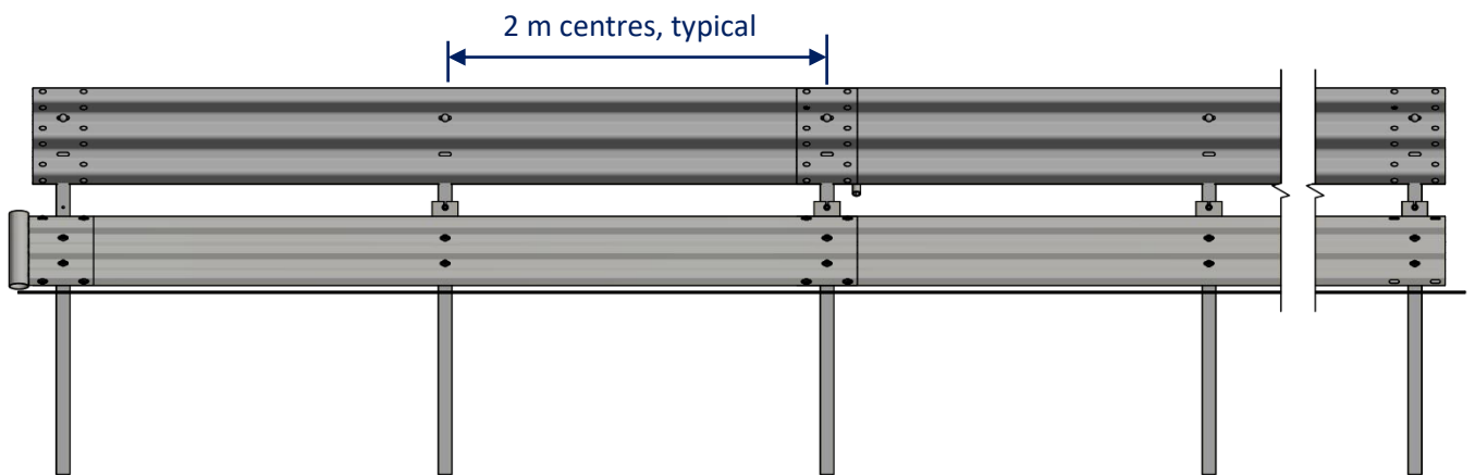
Attachment to Sentry Thrie-Beam FRONT VIEW
