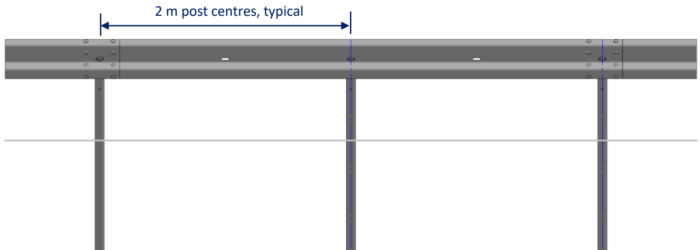
FRONT VIEW
