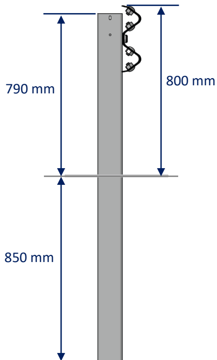
SIDE ELEVATION
