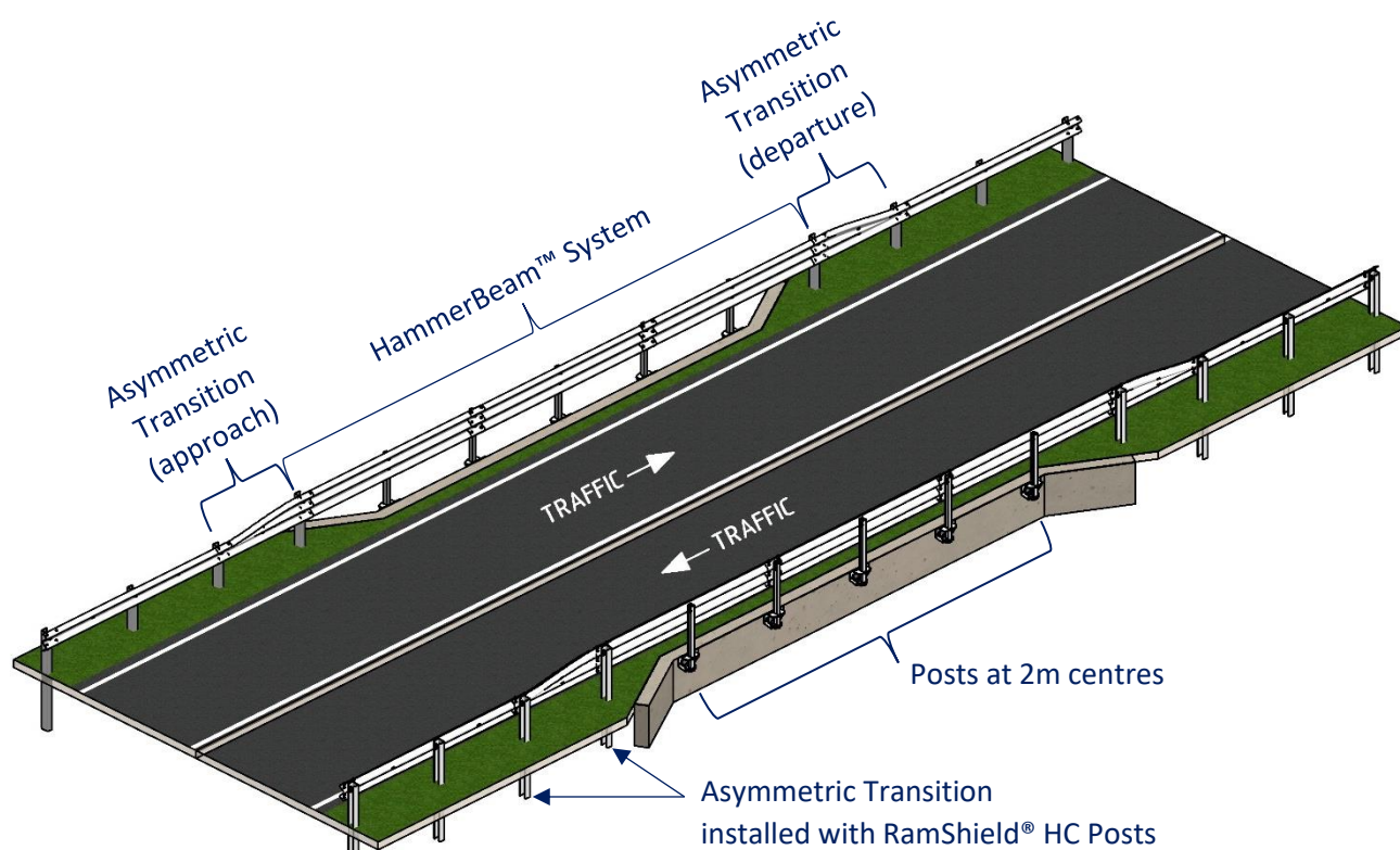
ASSEMBLY DETAIL
