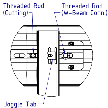
DETAIL B TYP. JOGGLE TAB/ THREADED ROD/ POST ARRANGEMENT SCALE 1:10
